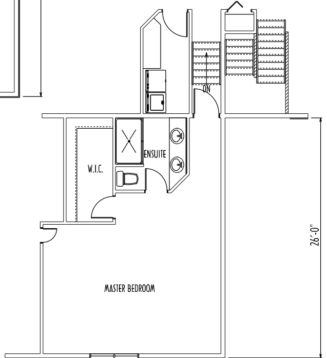
LOFT FLOOR PLAN LOFT FLOOR AREA 616 SQ. FT.
